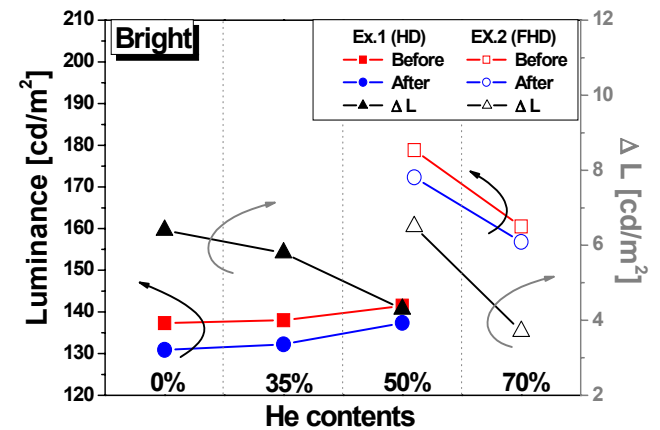
Fig. 8. Luminance and differences in luminance measured before and after discharge in region B on a bright screen with various He contents.
