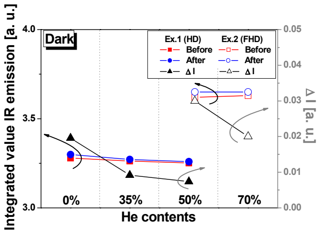
Fig. 6. Differences in the integrated value of the IR emission of region B in Fig. 5 during the reset period with various He contents.
