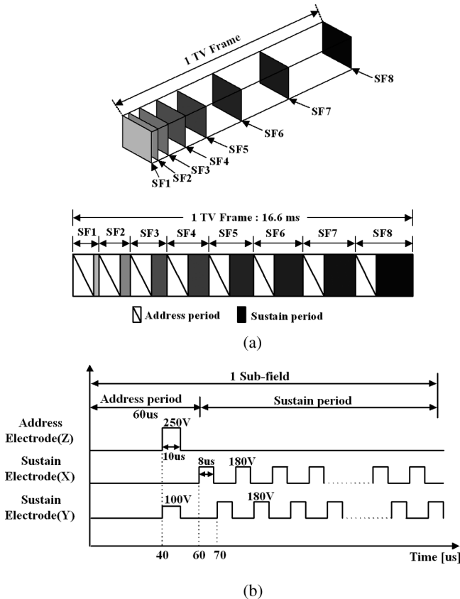
FIGURE 2 Sub-fields in single TV field (a) and timing diagram of voltage pulse waveforms (b) applied to three electrodes in one sub-field.
